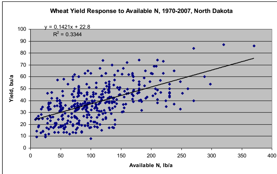
Figure 2. Spring wheat yield compared with N rate, 1970-2007. N Recommendation using this relationship is (N recommendation) = (7 X Yield Potential) – 160 – credits.
