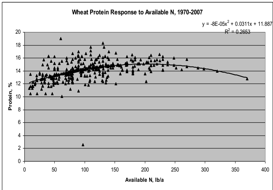
Figure 3. Spring wheat protein response with N-rate (total known available-N).
